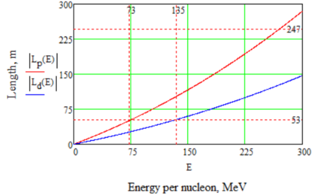
Fig. 2. Total length of spin compensator needed to make QFS lattice for deuteron and proton.
